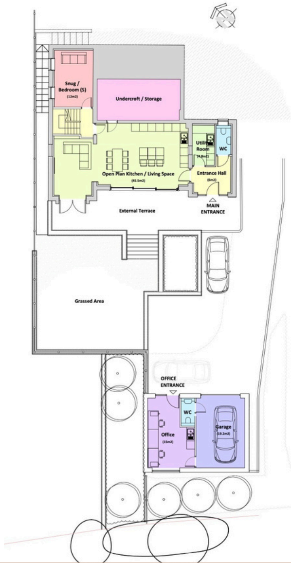
PROPOSED UPPER GROUND FLOOR PLAN - 1:100 (90m 2 )
